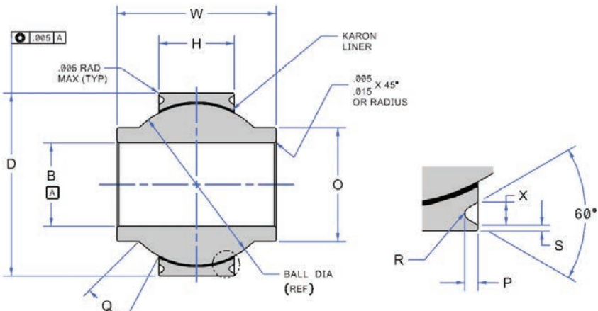
KR-CEG Series / Extended Inner Race, High Misalignment with Groove
