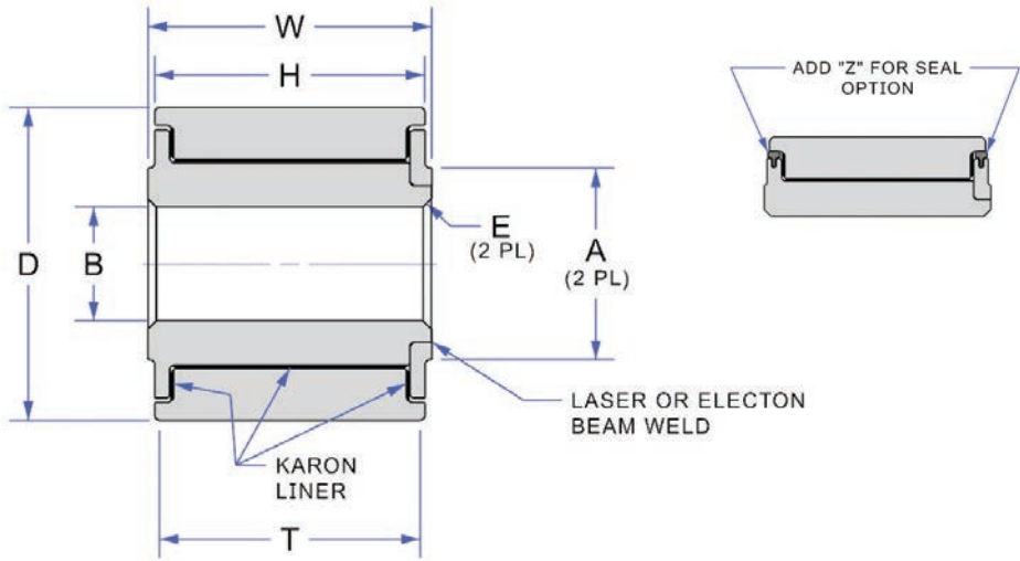
KRP523 / KRP 503 Series Heavy Duty Track Rollers
